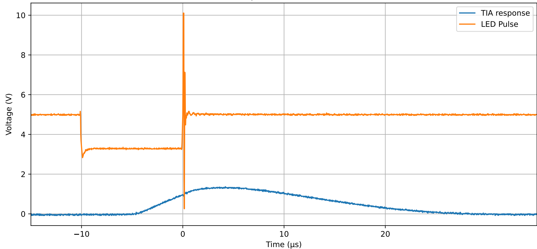
TIA circuit response to LED Pulse at 1 mm
